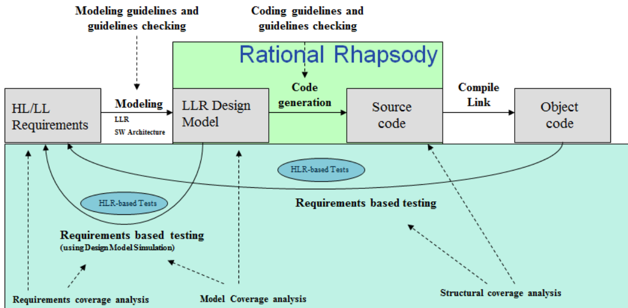
Figure 1: IBM Rational Rhapsody Reference Workflow
